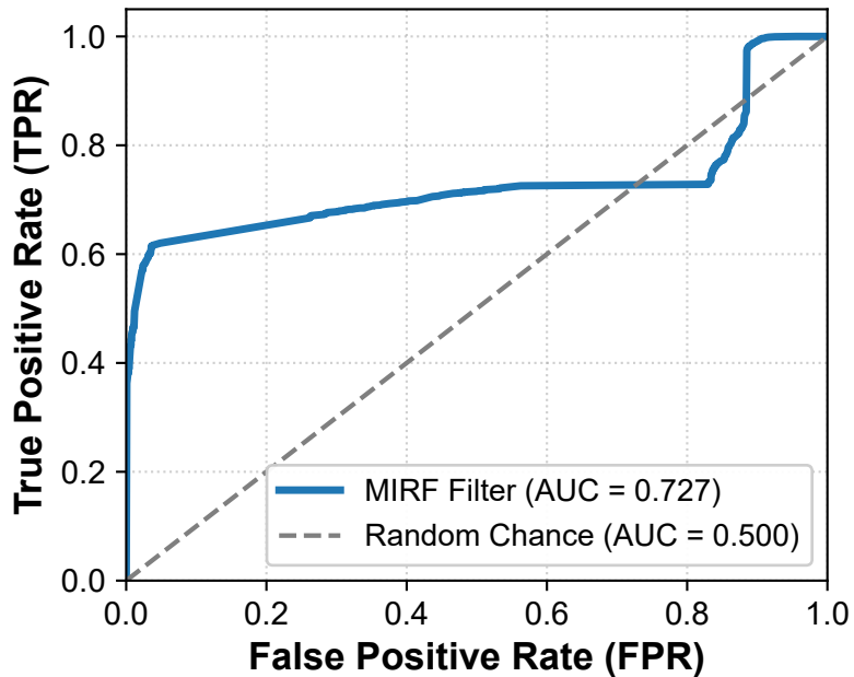
(a) Review-Bombing ROC Curve
