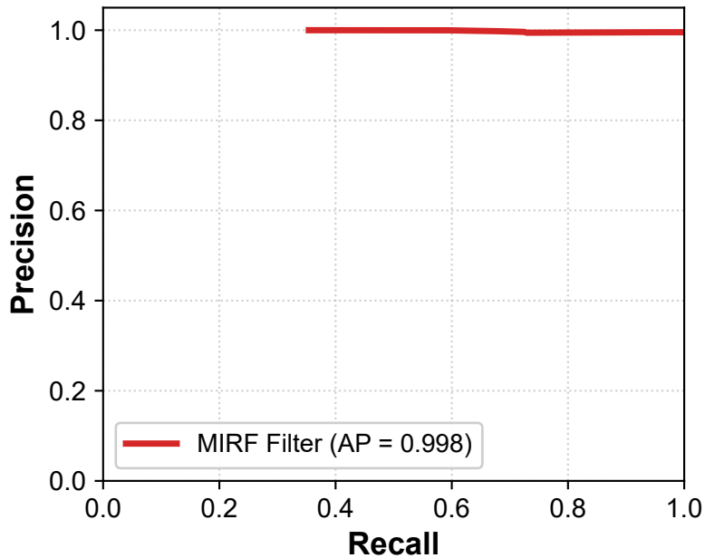
(b) Precision-Recall Curve
