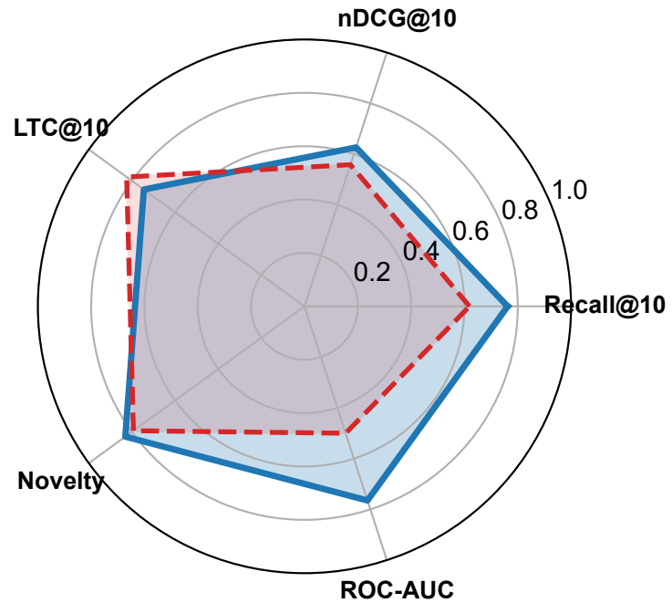
(c) Yelp (SGL)
