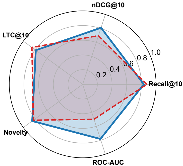
(b) Amazon (SimGCL)
