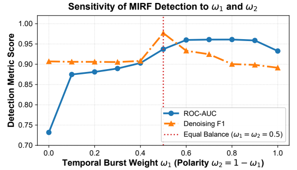
Figure 4: Sensitivity analysis of the MIRF detection F1-score and ROC-AUC with respect to temporal burst weight \omega_1 .
