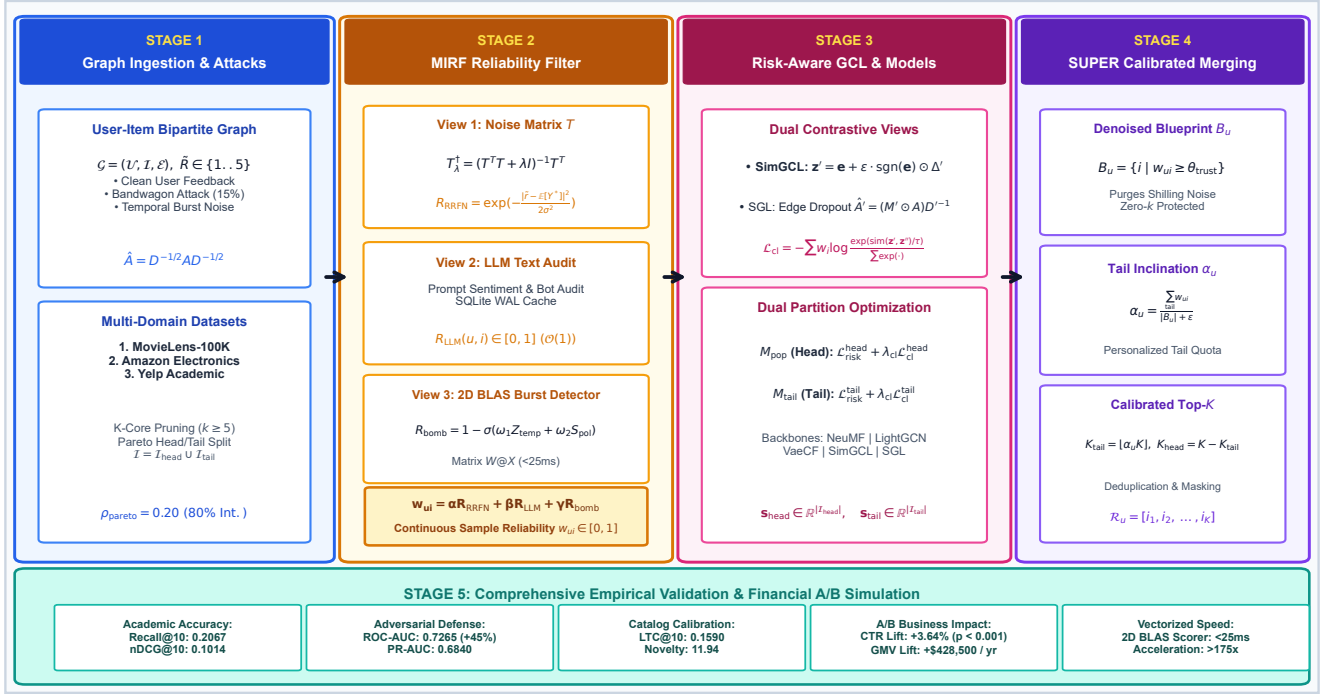
Figure 1: End-to-end system architecture of the RRFN-LLM-SUPER framework, illustrating data ingestion, noise transition modeling, the Multi-view Interaction Reliability Filter (MIRF), graph contrastive learning, dual partition training, and SUPER blueprint calibrated merging.
