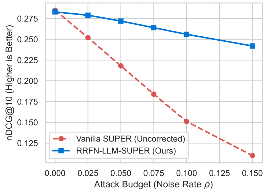
(a) Ranking Accuracy under Bandwagon Attack
