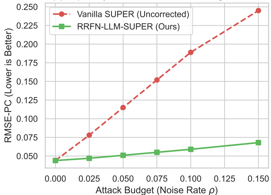
(b) Popularity Calibration under Bandwagon Attack
