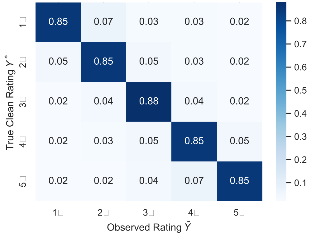
(b) Refined Transition Matrix T_{final} = \text{Softmax}(\hat{T} + \Delta T)
