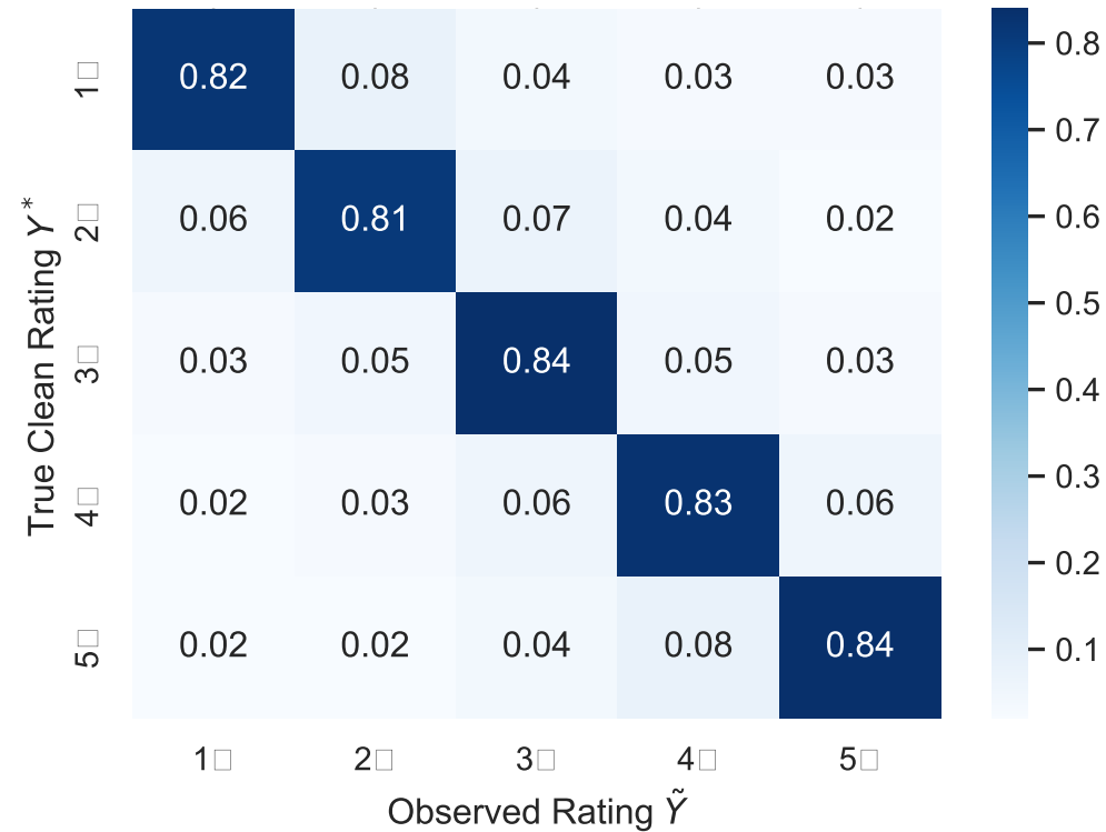
(a) Empirical Estimate \hat{T} (Anchor Points)
