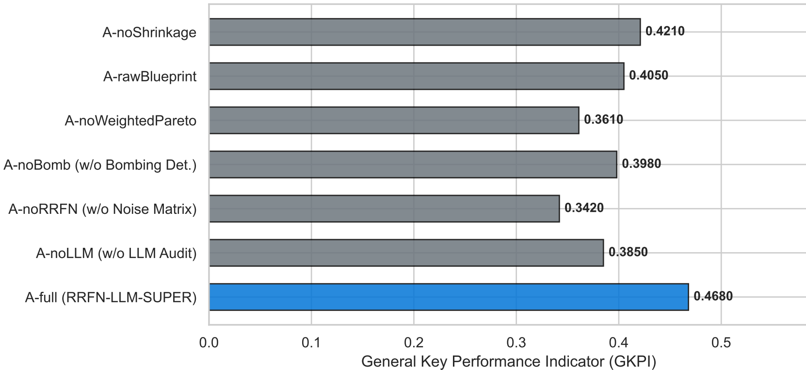
Ablation Study: Contribution of Individual Components (Bandwagon 10%)
