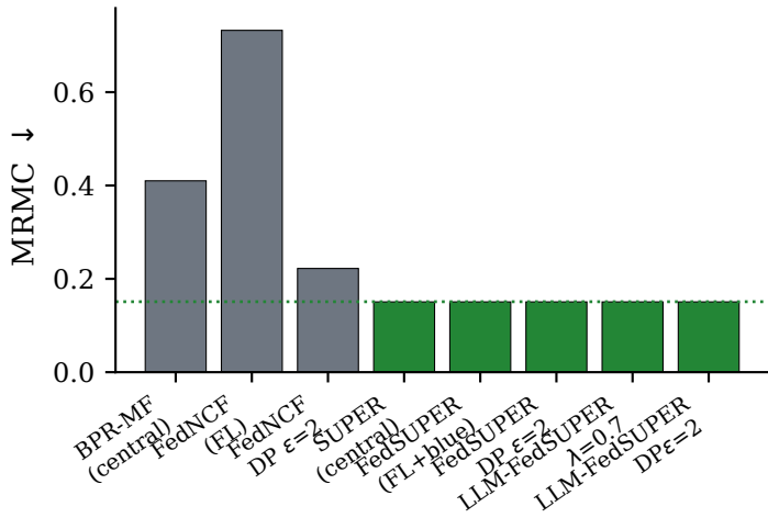
(b) Mean Rank Miscalibration
