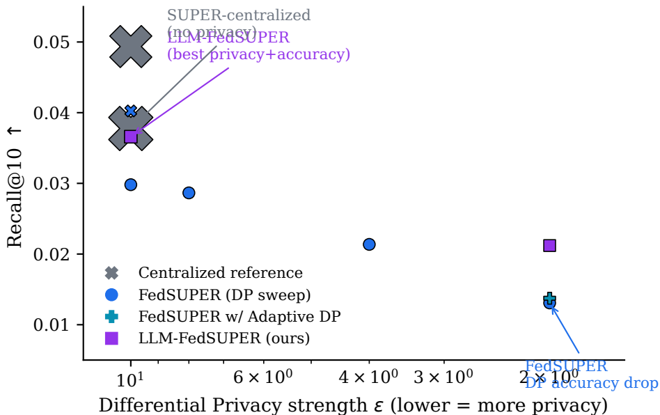
Accuracy-Privacy trade-off; marker size \propto Long-Tail Coverage (LTC)
