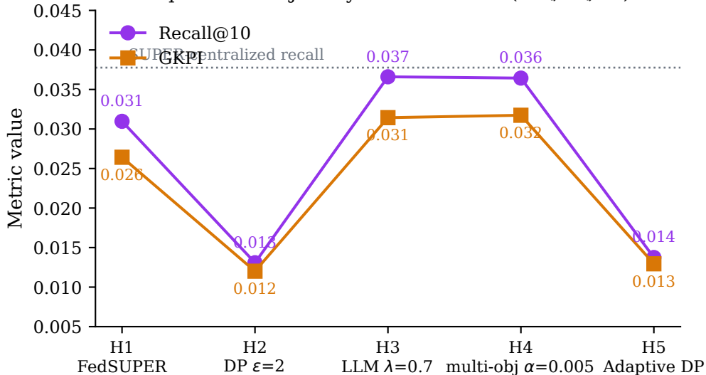
Experiment trajectory across 12 runs (H1\, \rightarrow \,H5)
