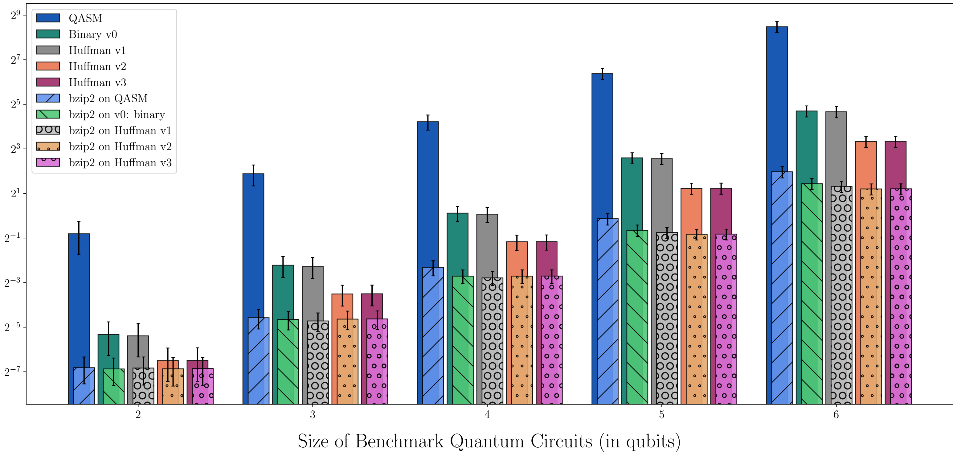
Average Program Size (in megabits)
