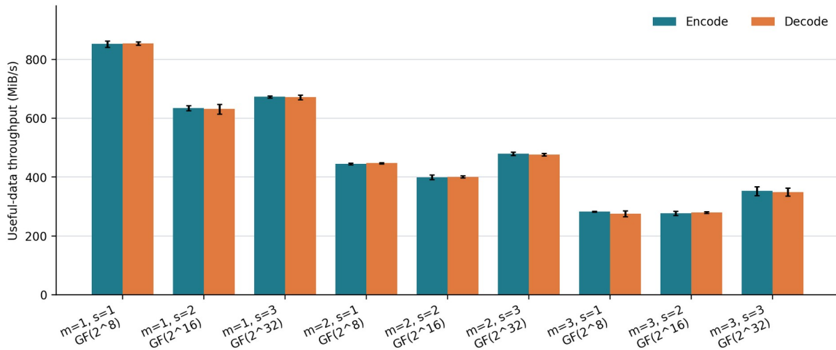
Figure 1. Mean sequential useful-data throughput; error bars show one standard deviation across ten trials.
