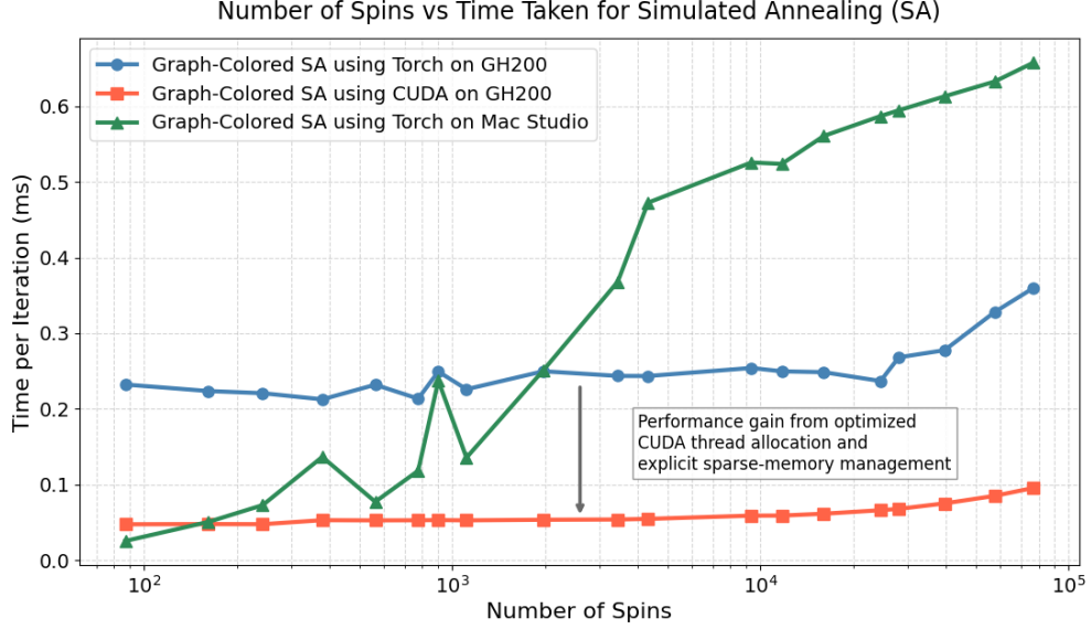
Fig. 4 SA wall-clock per sweep iteration versus number of Ising spins, comparing the CUDA kernel on GH200, a PyTorch implementation on GH200, and the same PyTorch code on an Apple M2 Max via Metal Performance Shaders (MPS)
