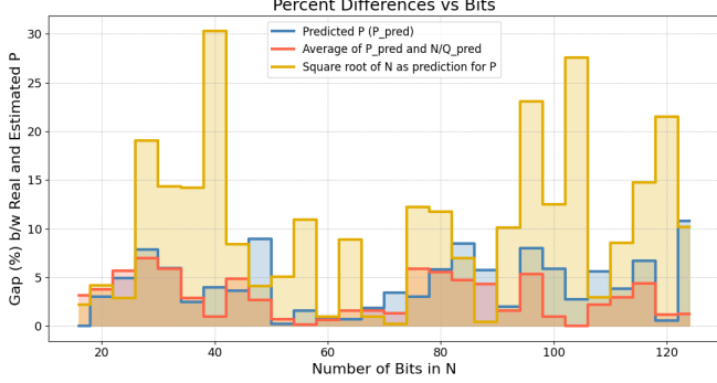
FIG. 6. Percentage gap between predicted and true P as a function of n , for three estimators: \sqrt{N} (uniform baseline), P_{\text{pred}} from SA, and the averaged centroid \frac{1}{2}(P_{\text{pred}} + N/Q_{\text{pred}}) . Means across the tested range: 10.33% for \sqrt{N} , 4.23% for raw SA, and 2.98% for the centroid.
