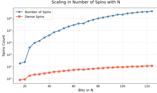
FIG. 2. Number of total Ising spins versus number of densely connected hub spins as the bit width of N grows to \sim 128 . Total grows as \mathcal{O}(n^3) ; hub count grows as \mathcal{O}(\log N) .
