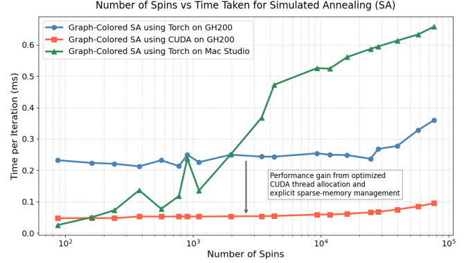
FIG. 4. SA wall-clock per sweep iteration versus number of Ising spins, comparing the CUDA kernel on GH200, a PyTorch implementation on GH200, and the same PyTorch code on an Apple M2 Max via MPS. CUDA stays near 0.05 ms across four decades of spin count; the PyTorch variants drift upward past 10^3 spins.
