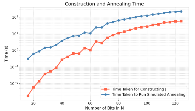
FIG. 5. Time to build J and time to run one full annealing schedule, both as a function of n in [16, 128] bits. Construction is sub-second up to \sim 60 bits and reaches \sim 60 s at 128 bits. Annealing dominates above \sim 60 bits, reaching \sim 220 s at 128 bits.
