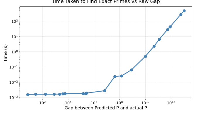
FIG. 7. Time taken to find the exact factor by the wheel-sieve brute-force search, as a function of the raw gap between P_{\text{centre}} and the true P , on the 72-thread GH200 Grace CPU. For small gaps the whole search fits in a single parallel pass across the threads, so the time is roughly constant; once the gap exceeds what 72 threads can cover in one pass the search effectively goes serial and the time climbs linearly, following the \text{Gap} \cdot 2^n model of Eq. (8).
