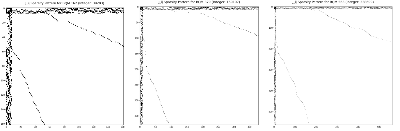
FIG. 1. Sparsity of J_{ij} at N = 39\,203 (162 spins), 159\,197 (379), and 338\,699 (563). Most nonzeros concentrate in a small band along the top rows / left columns, with a thin diagonal trail. Pattern persists across orders of magnitude in N .
