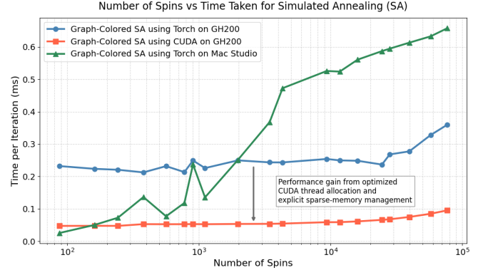
FIG. 4. SA wall-clock per sweep iteration versus number of Ising spins, comparing the CUDA kernel on GH200, a PyTorch implementation on GH200, and the same PyTorch code on an Apple M2 Max via MPS.
