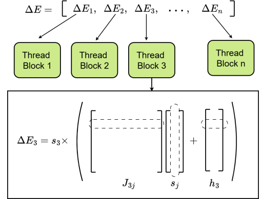
FIG. 3. Local-field evaluation of \Delta E_i . Each thread group loads spin i 's neighbour row from the CSR, multiplies each coupling J_{ij} by the neighbour spin \sigma_j , reduces the products to the local field L_i = \sum_j J_{ij} \sigma_j + h_i , and returns \Delta E_i = -2\sigma_i L_i . One group per spin lets all N differences be evaluated in a single parallel pass.
