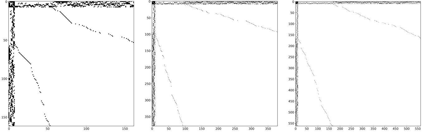
FIG. 1. Sparsity of J_{ij} at N = 39\,203 (162 spins), 159\,197 (379), and 338\,699 (563). Most nonzeros concentrate in a small band along the top rows / left columns, with a thin diagonal tail. This pattern persists across all orders of magnitude in N .
