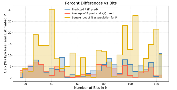
FIG. 6. Percentage gap between predicted and true P as a function of n , for three estimators: \sqrt{N} (baseline), P_{\text{pred}} from SA, and the averaged centroid \frac{1}{2}(P_{\text{pred}} + N/Q_{\text{pred}}) .
