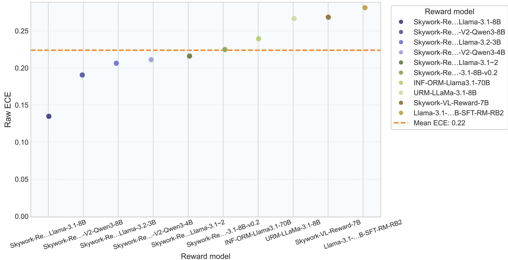
ECE scores (Top 10 by ECE)
