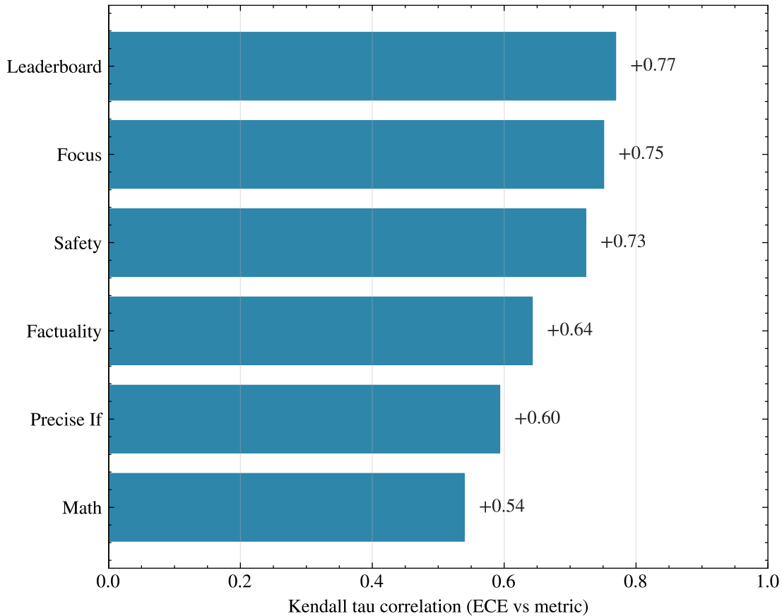
Correlation between ECE and RewardBench metrics
