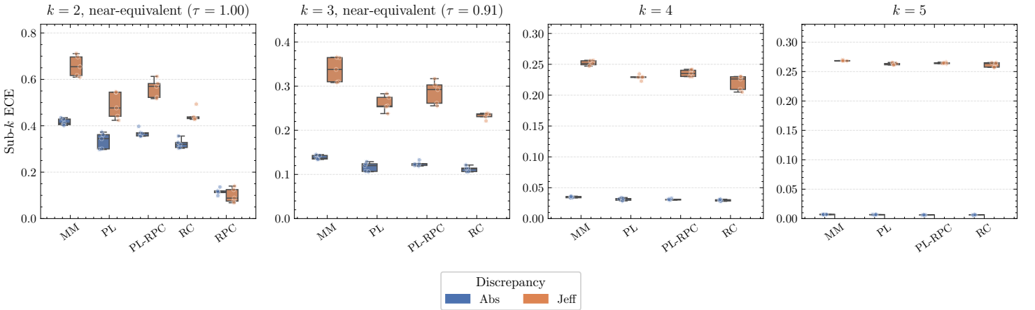
Figure 1: Comparison of using |\cdot| in contrast to Jeffrey Divergence for calculating sub- k calibration via ECE. Rank correlation of the methods is reported only if the values using |\cdot| are significantly different.
