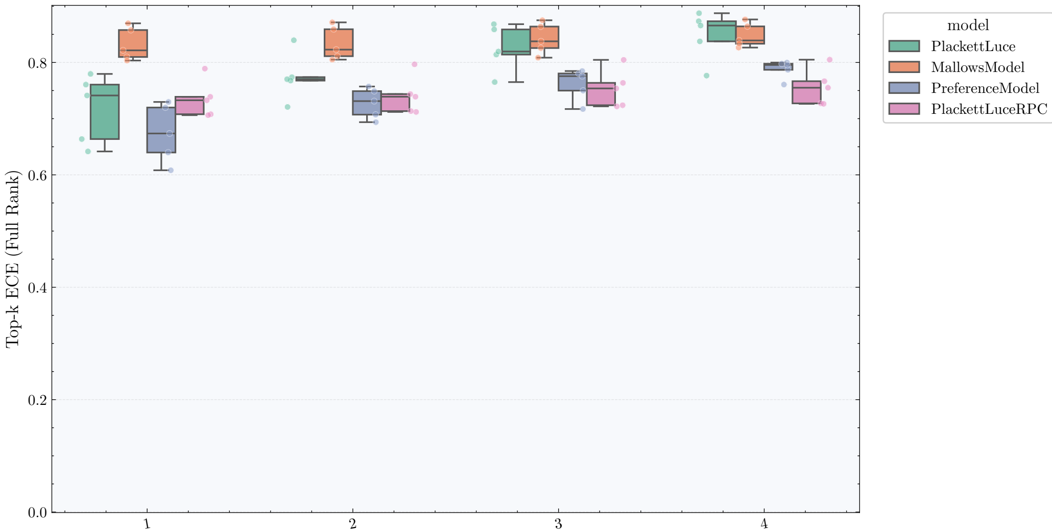
Top-k ECE per model on political (Full Rank)
