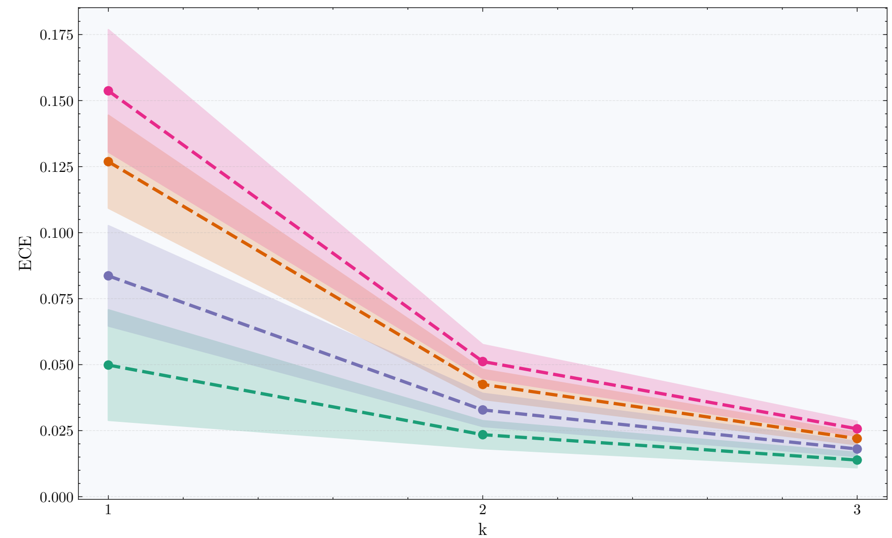
Top-k ECE vs k (Full Rank)
