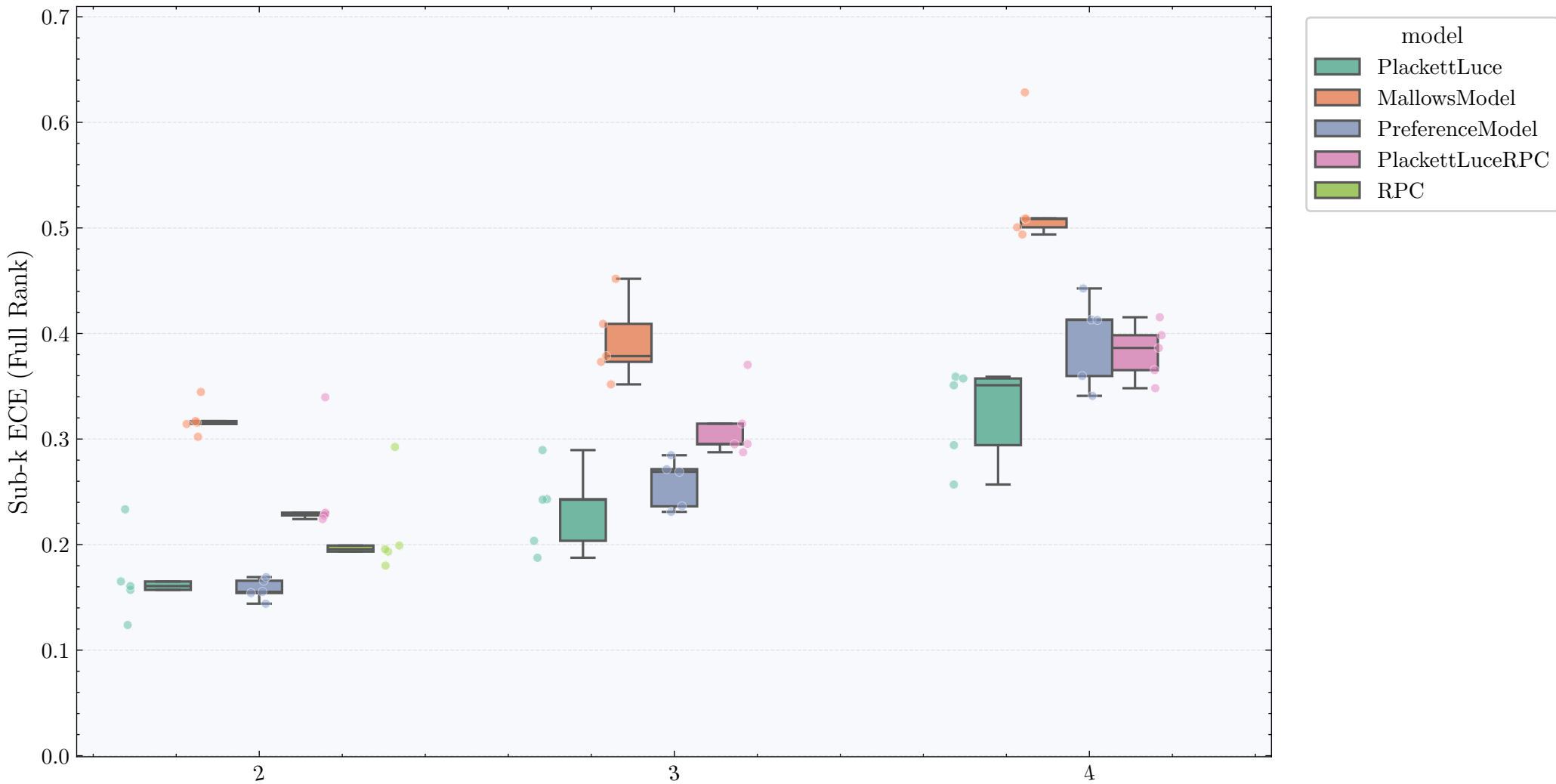
Sub-k ECE per model on authorship (Full Rank)
