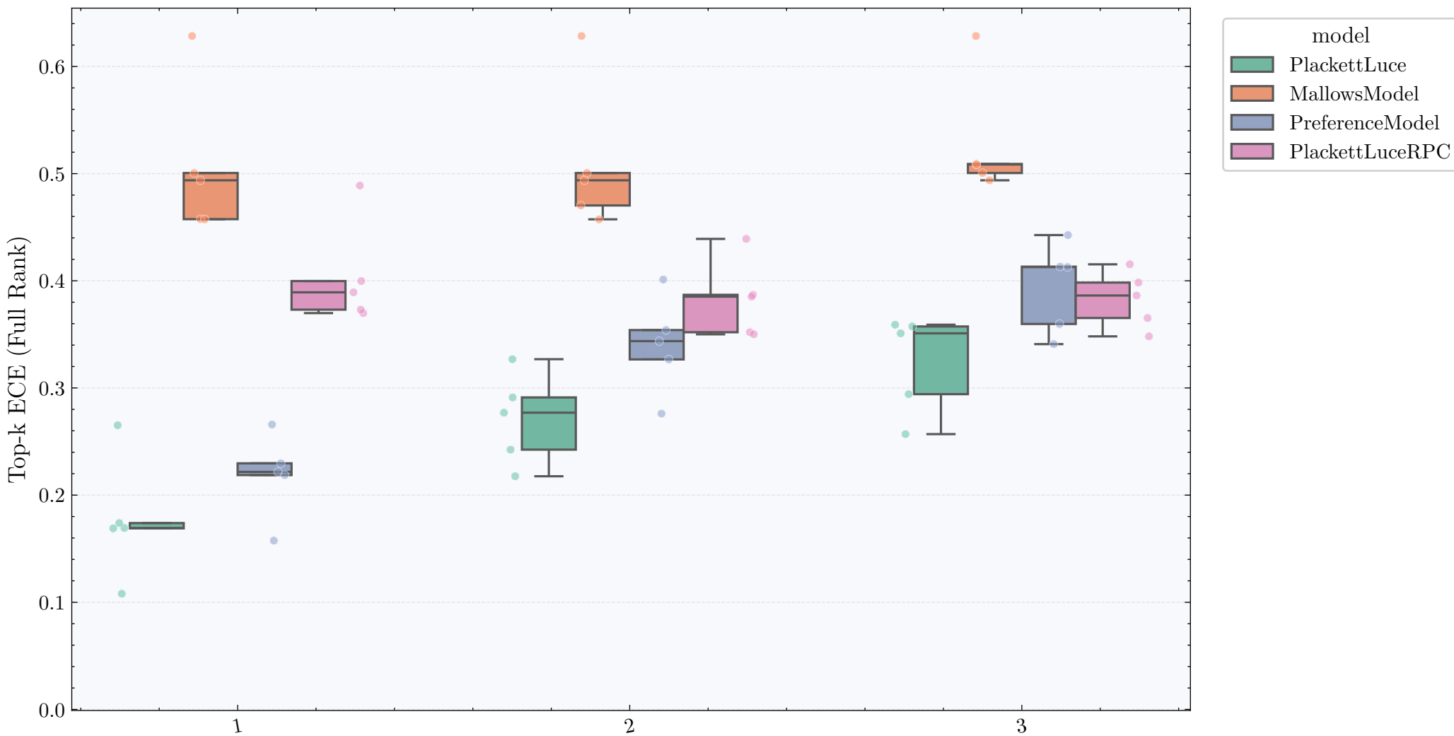
Top-k ECE per model on authorship (Full Rank)
