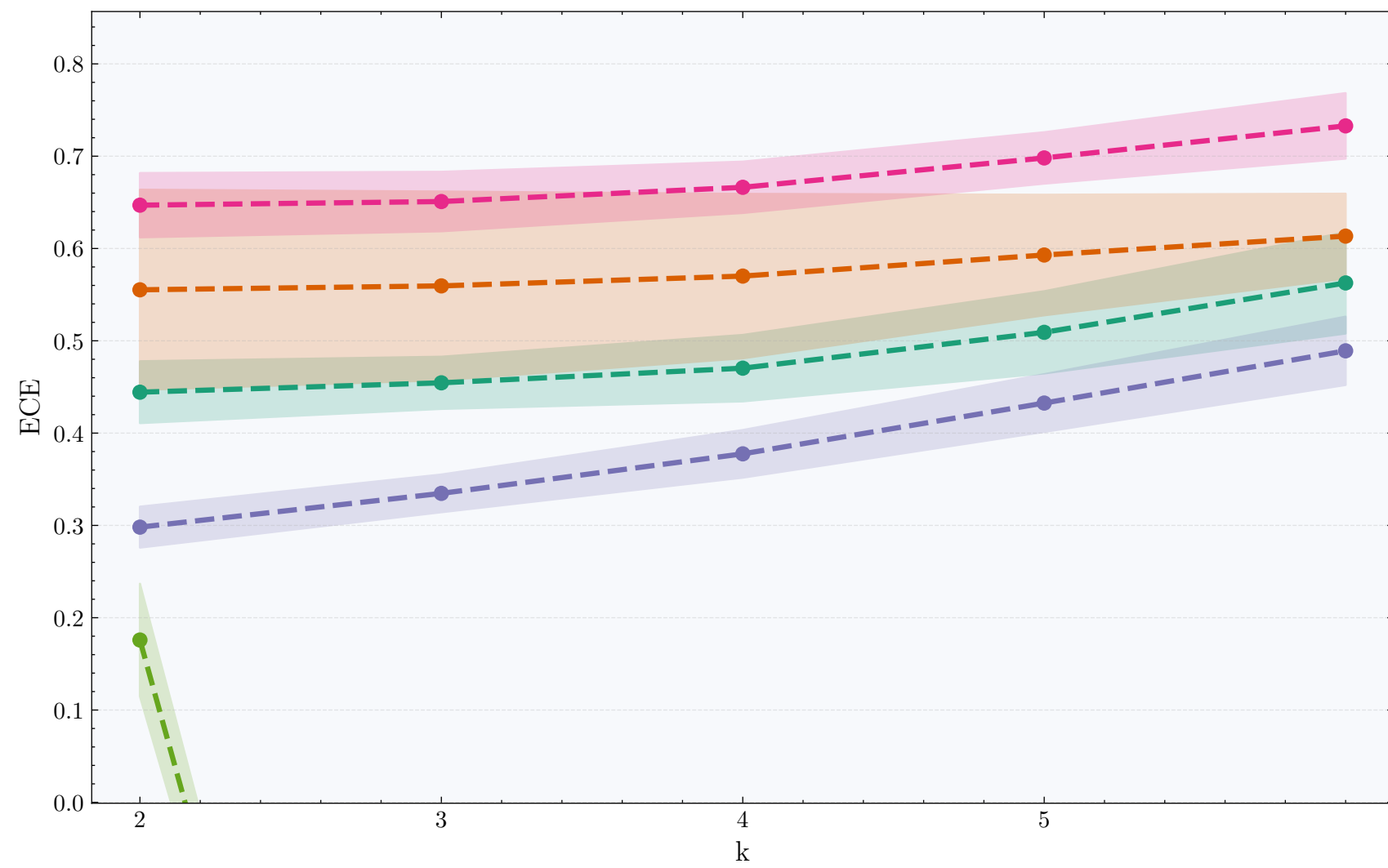
Sub-k ECE vs k (Full Rank)
