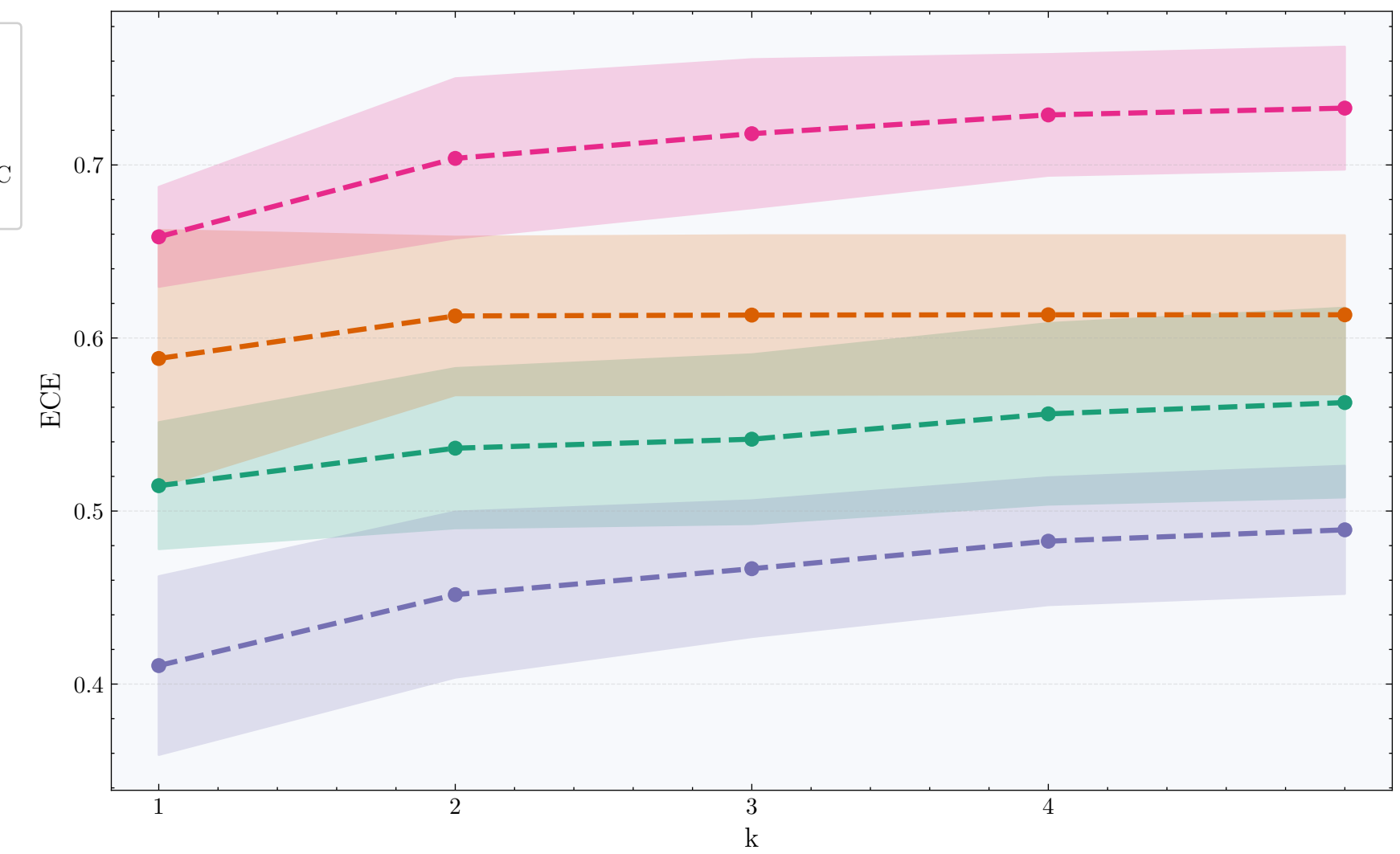
Top-k ECE vs k (Full Rank)
