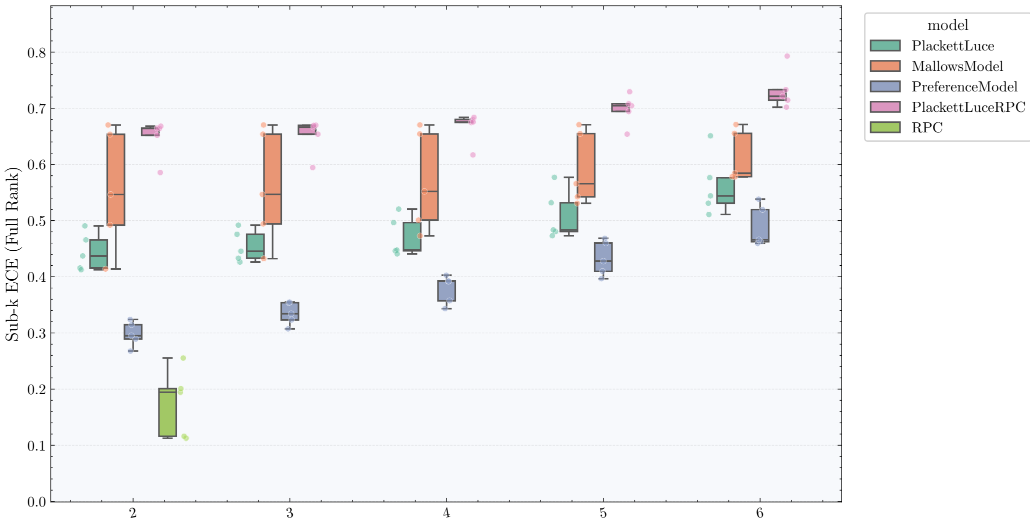
Sub-k ECE per model on glass (Full Rank)
