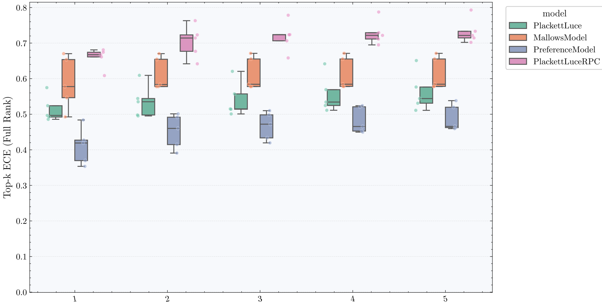
Top-k ECE per model on glass (Full Rank)
