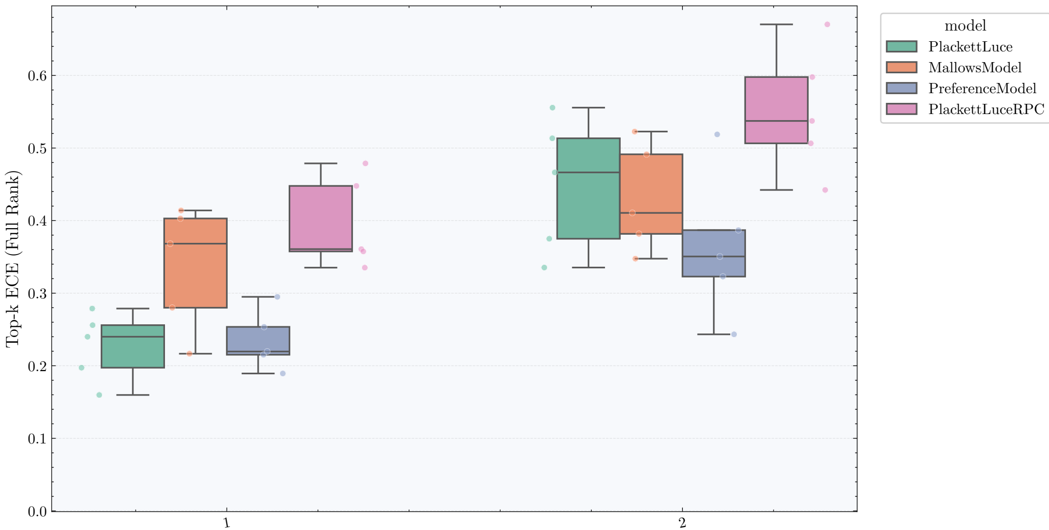
Top-k ECE per model on iris (Full Rank)
