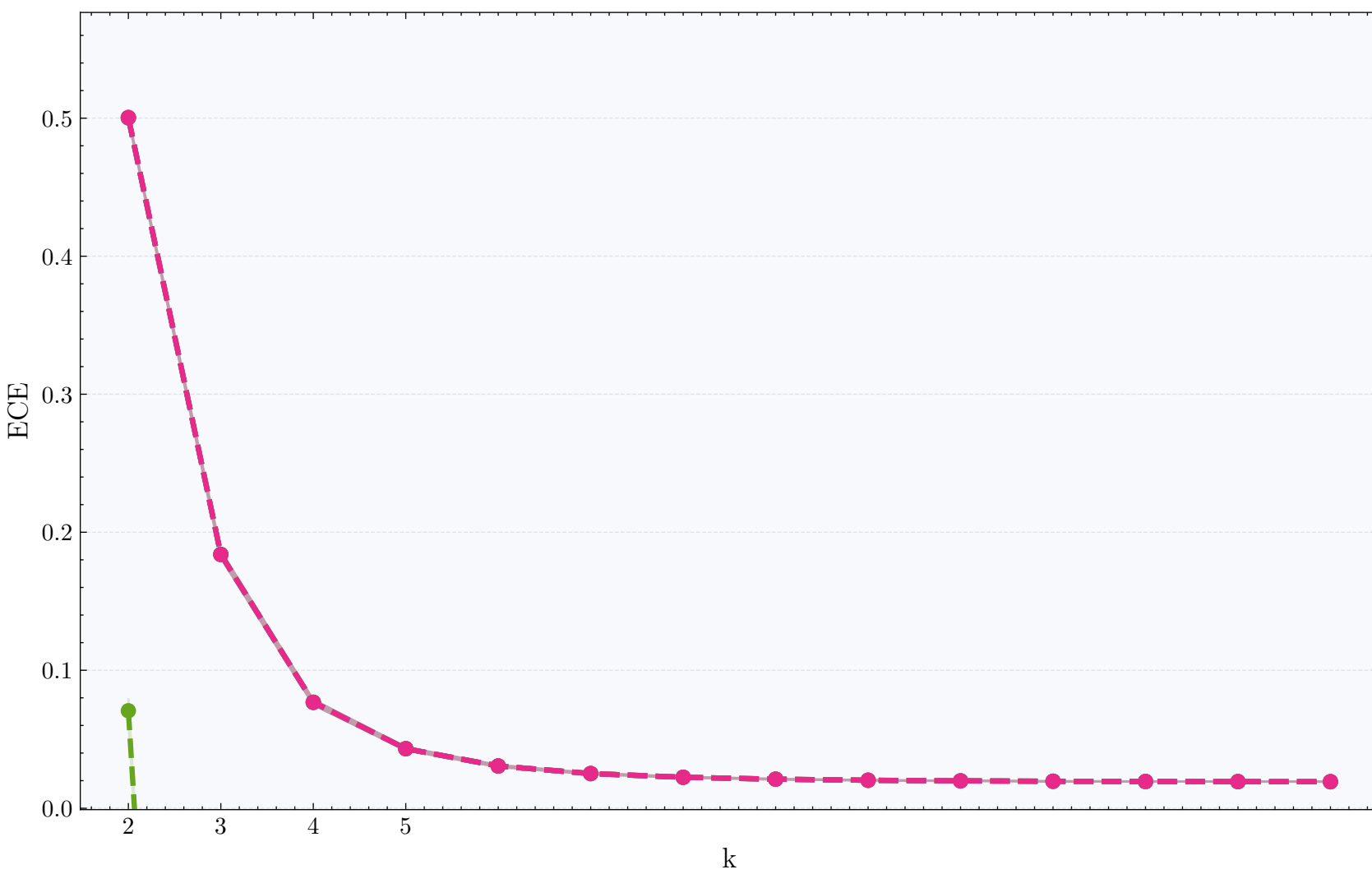
Sub-k ECE vs k (Full Rank)
