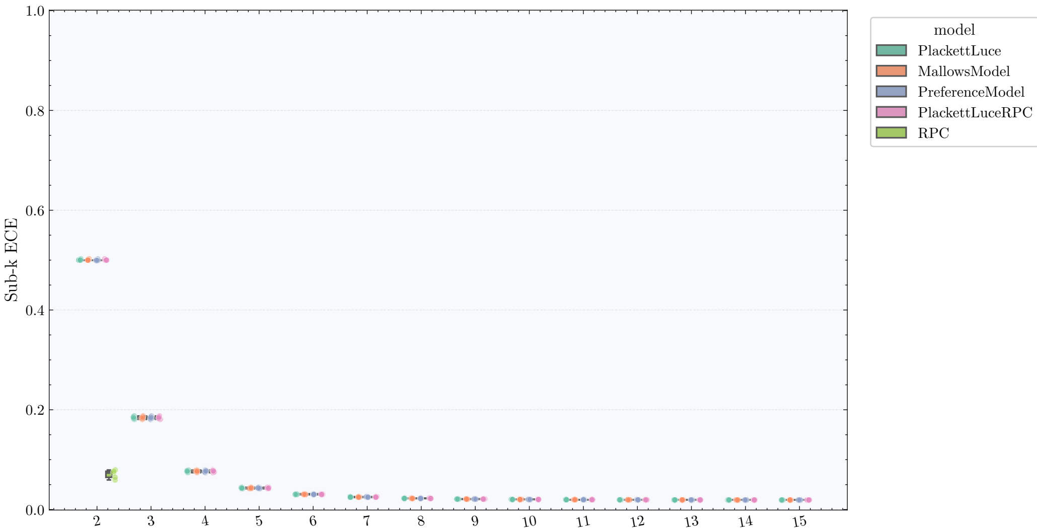
Sub-k ECE per model on movies
