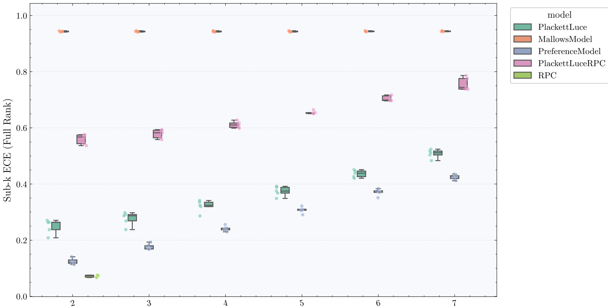
Sub-k ECE per model on segment (Full Rank)
