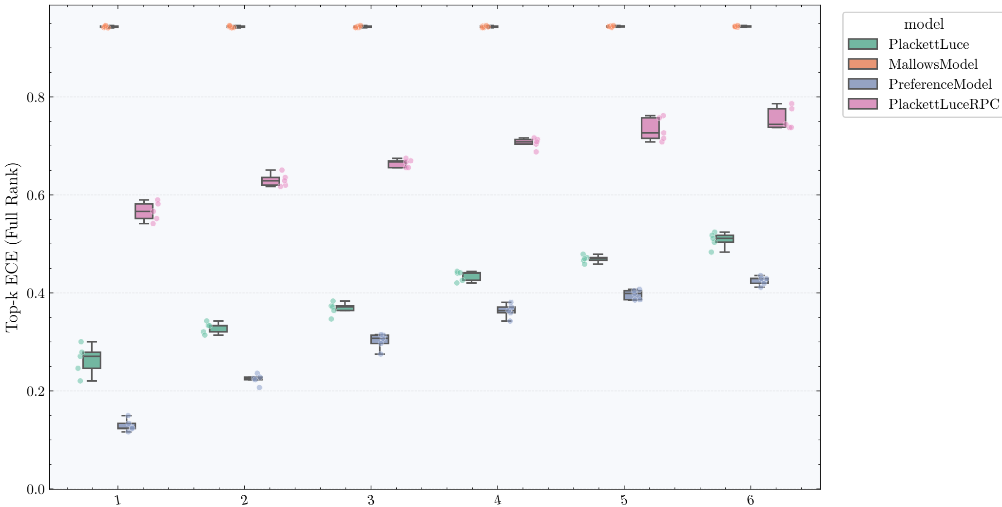
Top-k ECE per model on segment (Full Rank)
