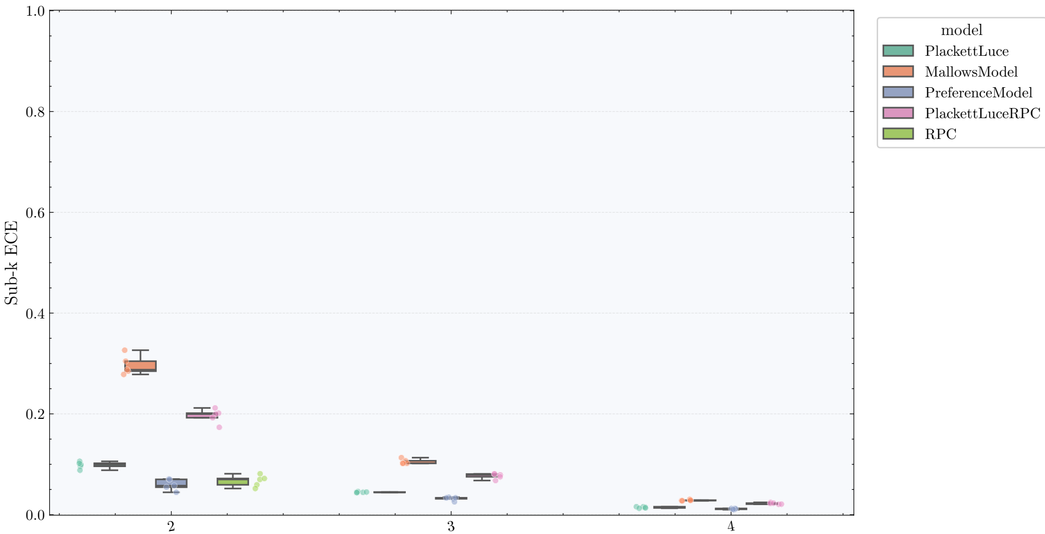
Sub-k ECE per model on vehicle
