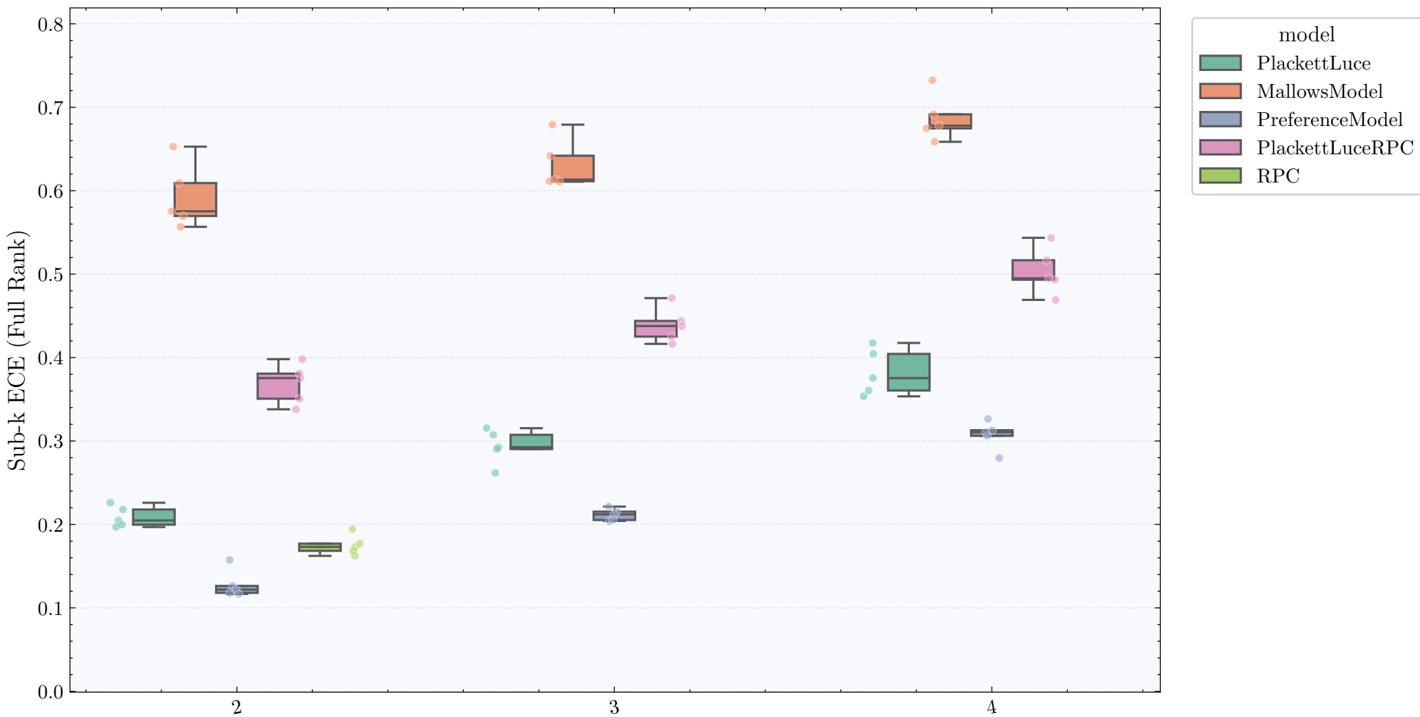
Sub-k ECE per model on vehicle (Full Rank)
