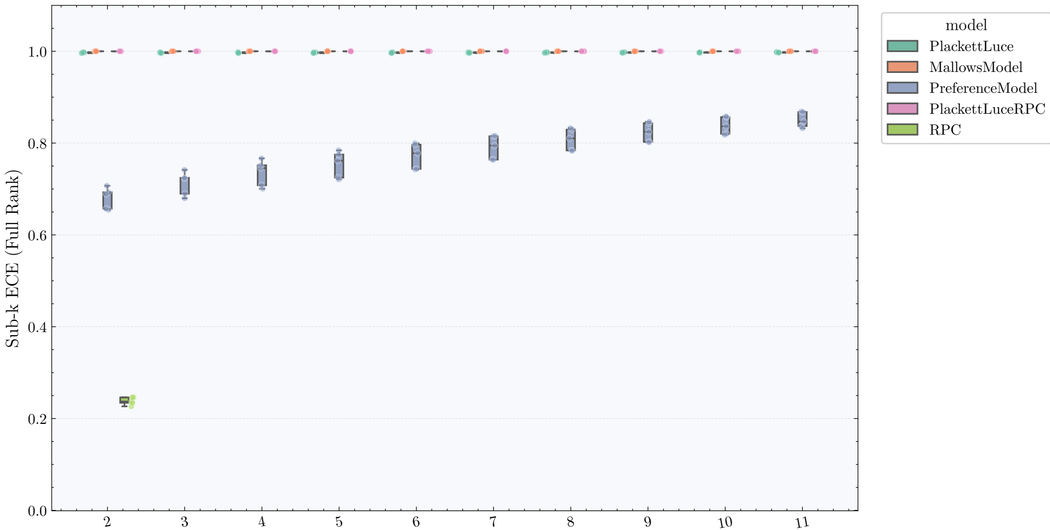
Sub-k ECE per model on vowel (Full Rank)
