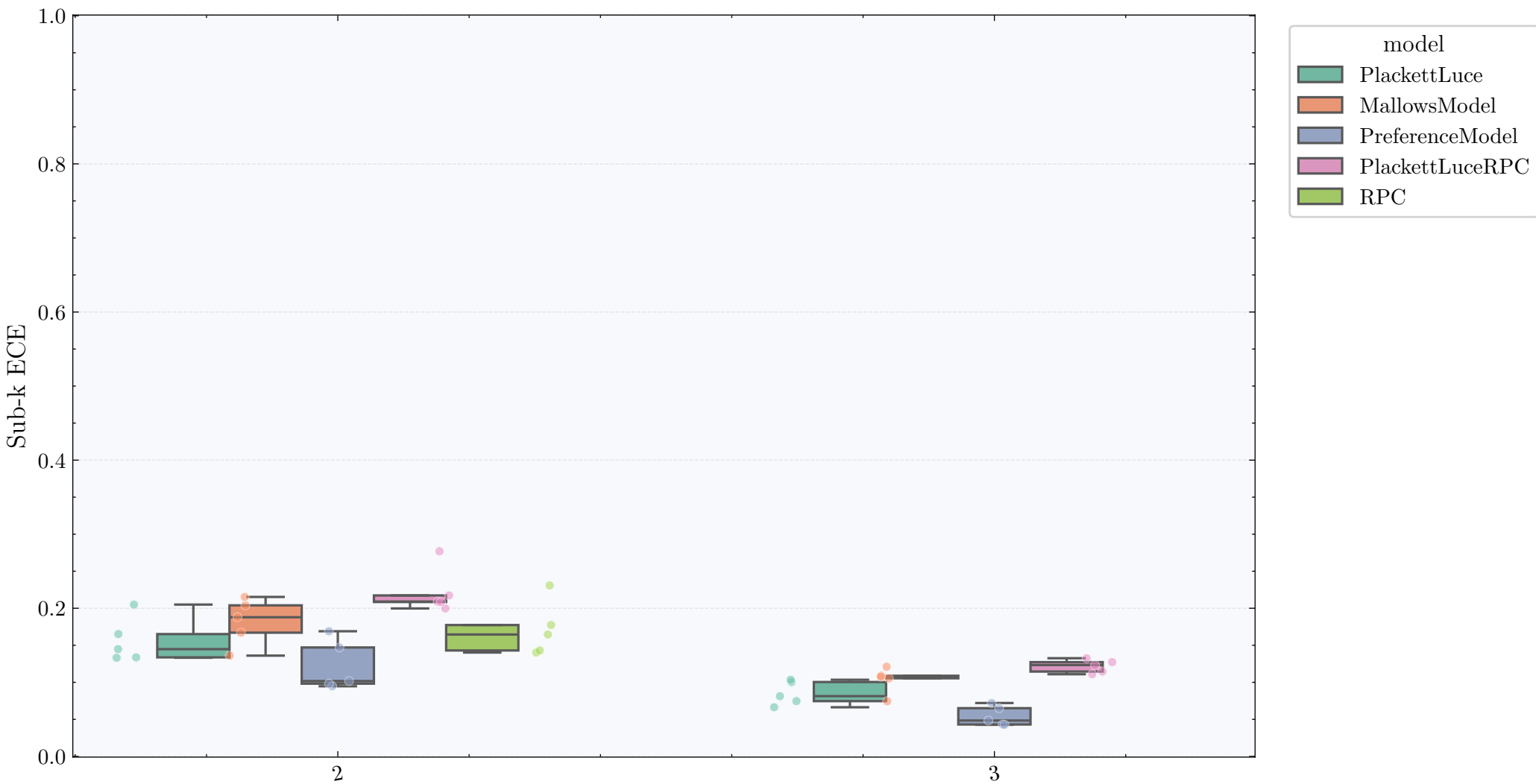
Sub-k ECE per model on wine
