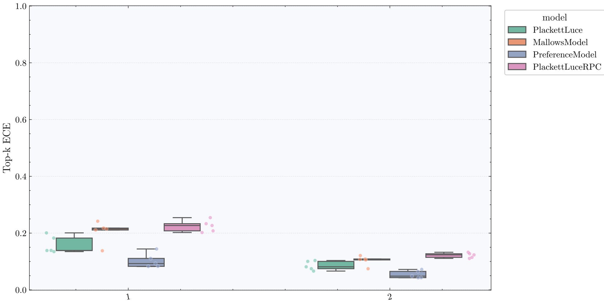
Top-k ECE per model on wine
