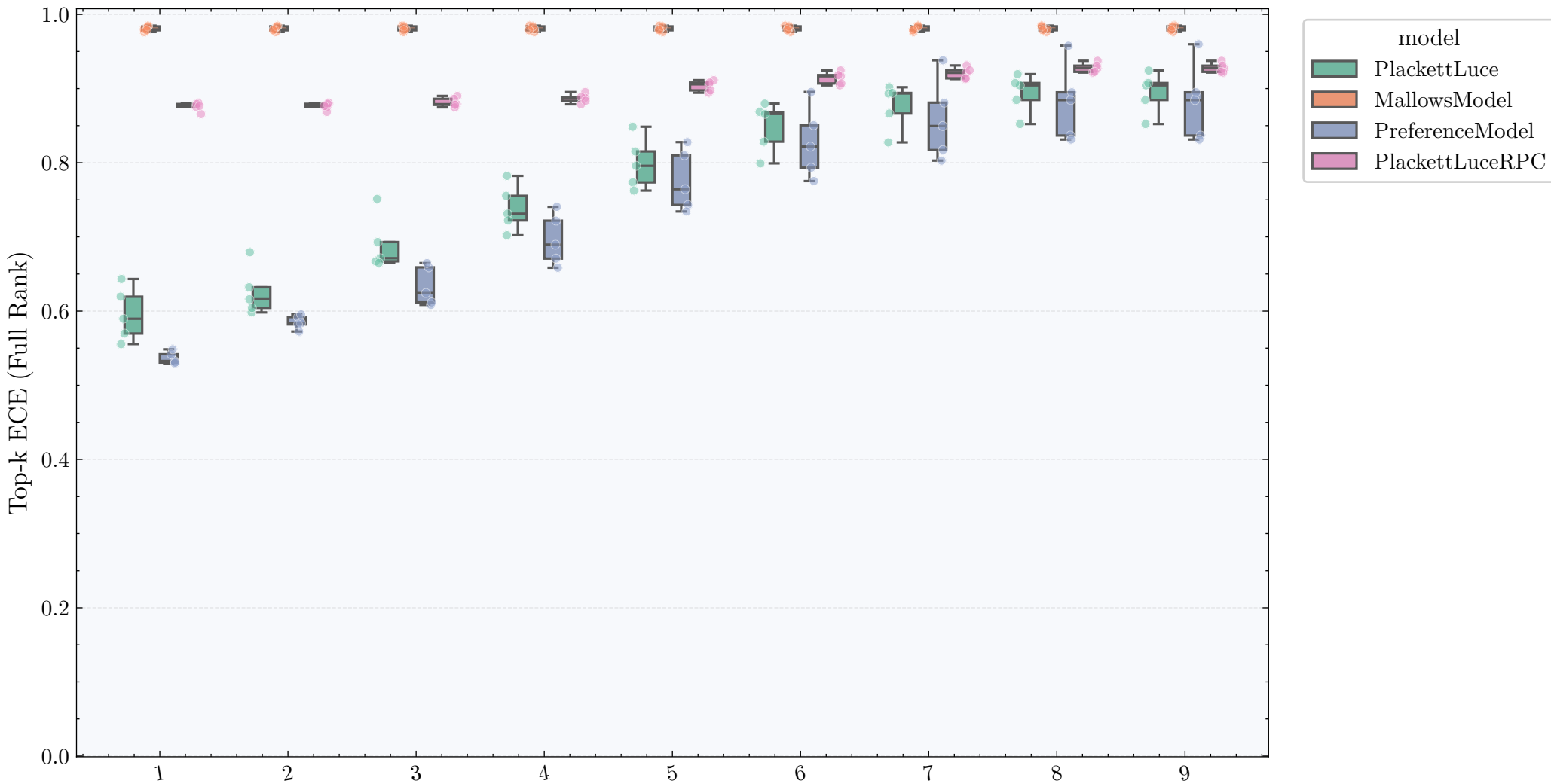
Top-k ECE per model on yeast (Full Rank)
