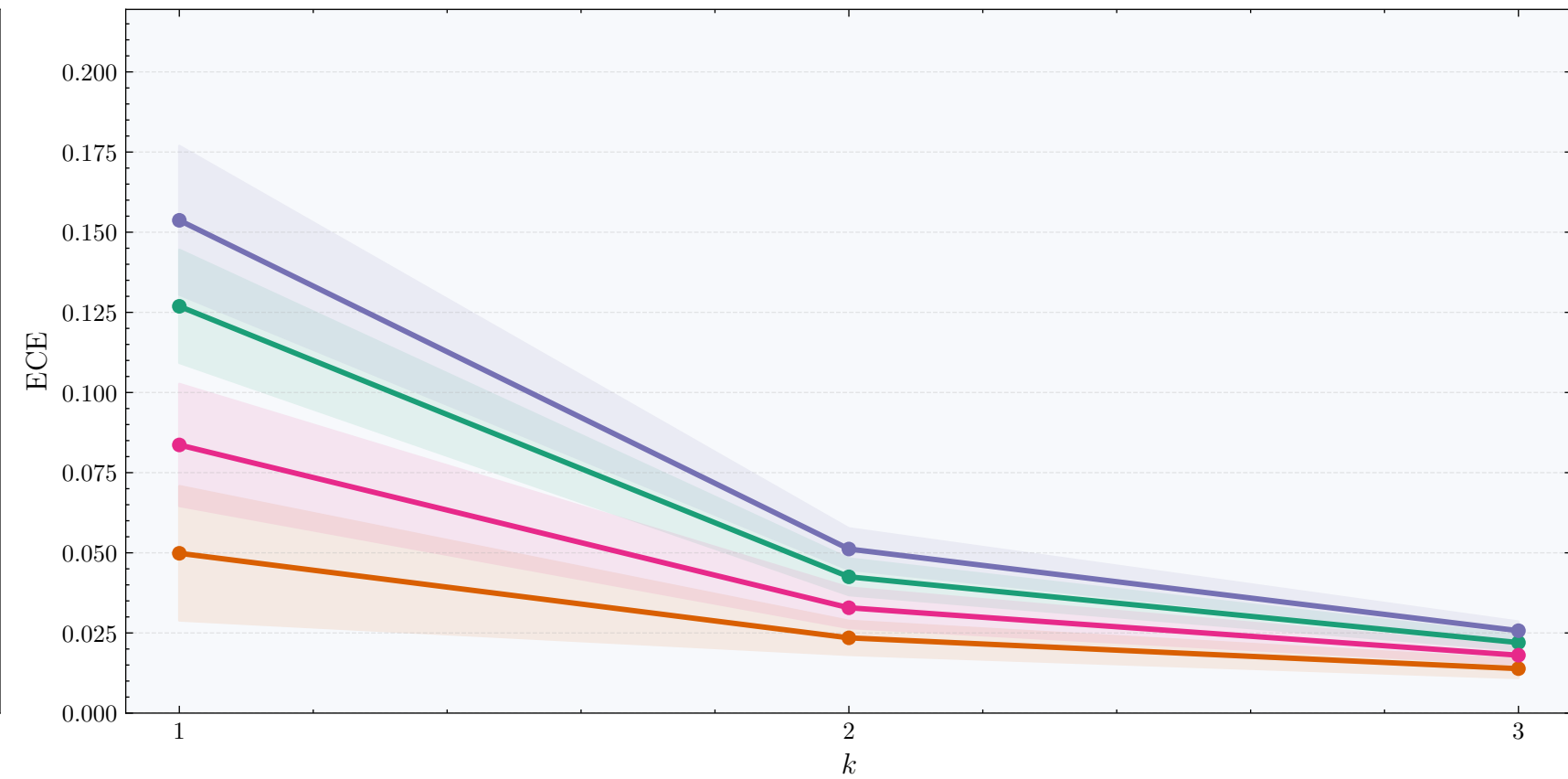
Top- k ECE (Full Rank) vs k
