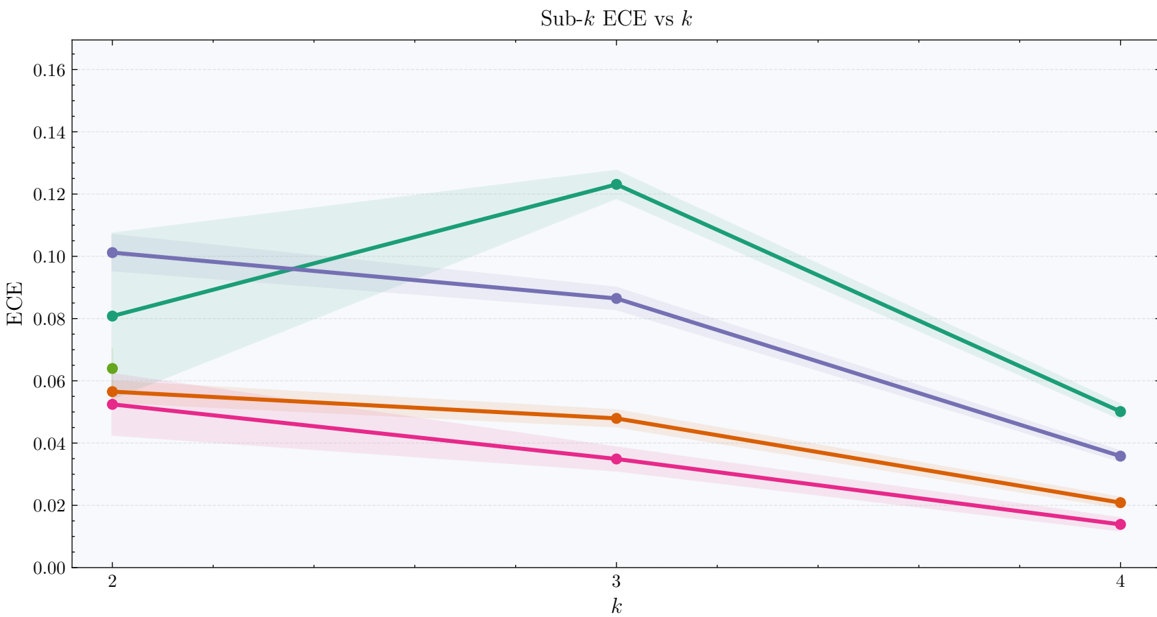
ECE vs k — vehicle
