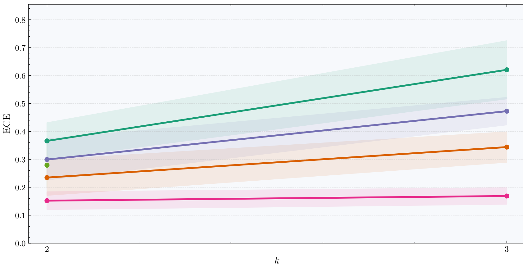
Sub- k ECE (Full Rank) vs k
