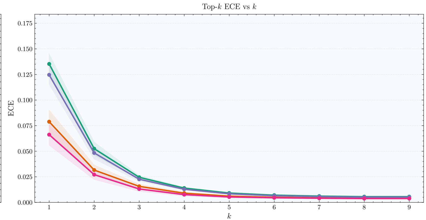
ECE vs k — yeast
