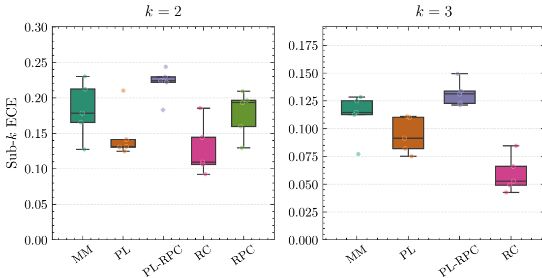
Model
