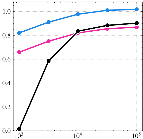
FIxLIP: ViT16
