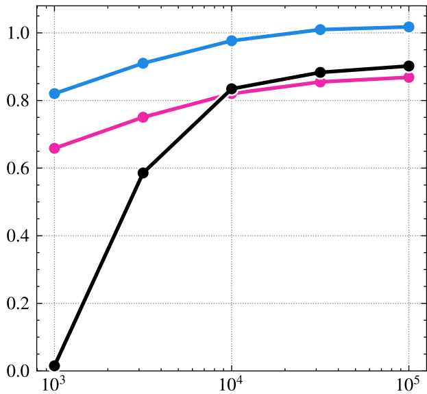
FIxLIP: ViT16
