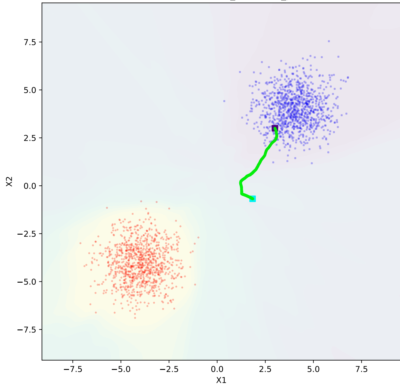
bubbles - connected_reference_point
