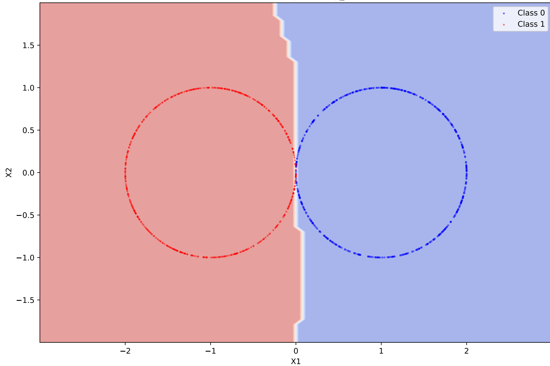
Decision Boundary - infinity_dataset
