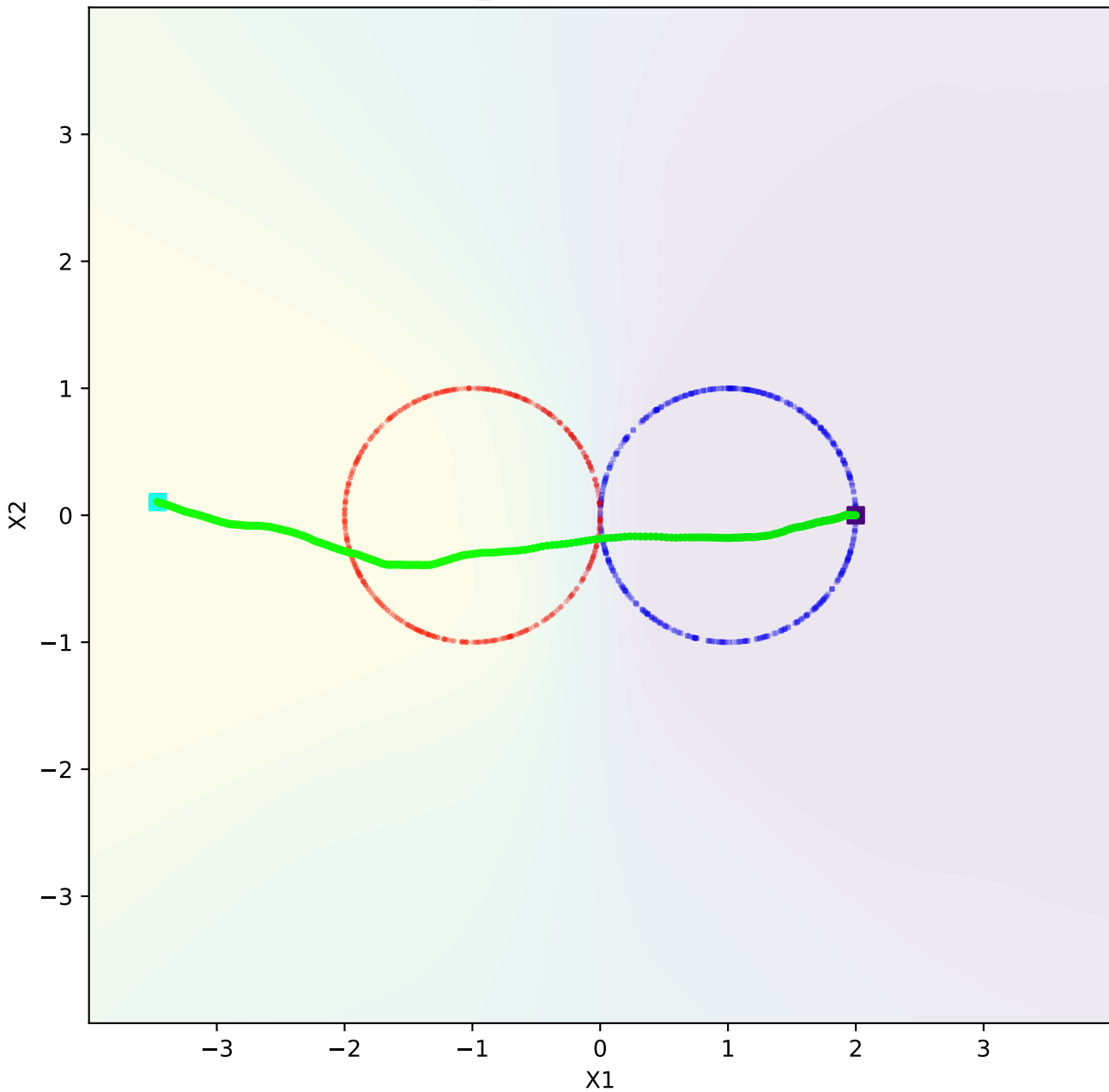
infinity_dataset - discriminative
