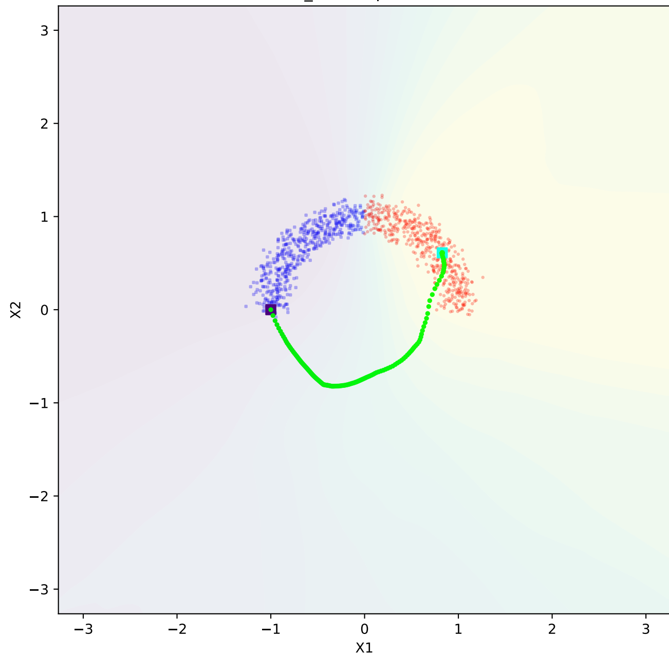
one_moon - plausible
