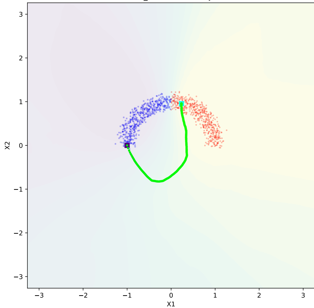
one_moon - similarity
