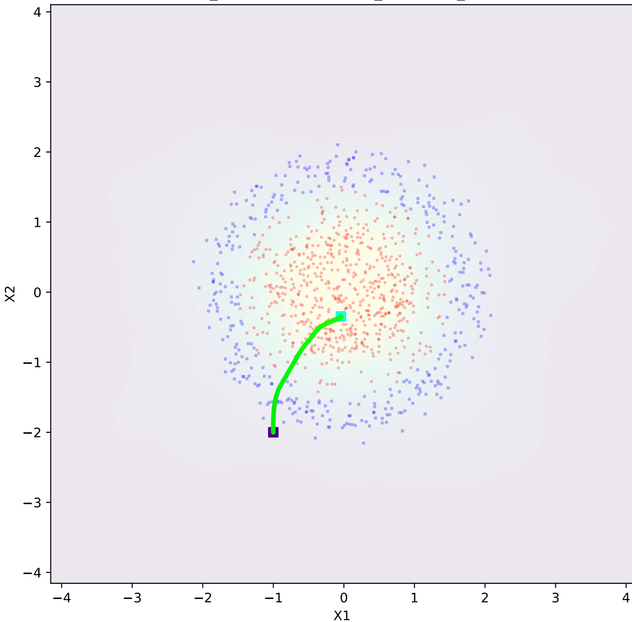
ring_dataset - connected_reference_point
